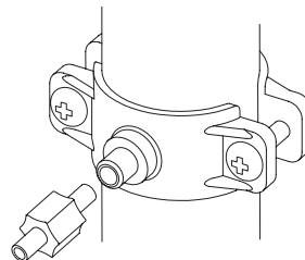
Figure 9b. Drain saddle installation
