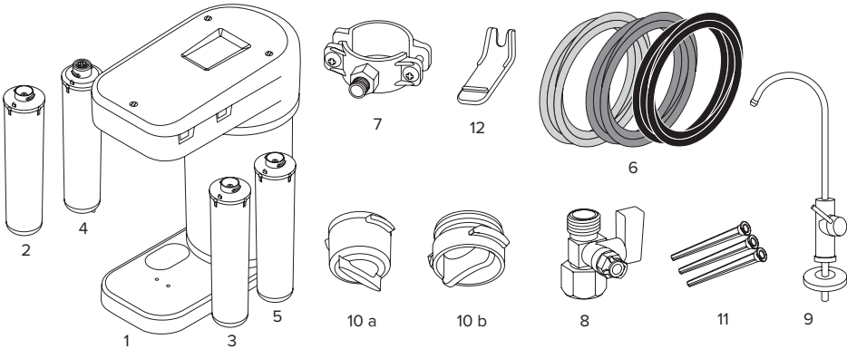
Figure 1. Product assembly
