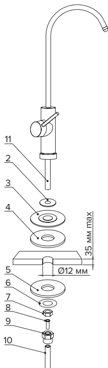
Figure 8. Tube connecting to the clean water faucet procedure
