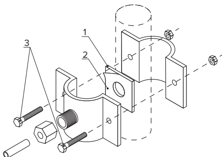
Figure 9a. Drain saddle components
